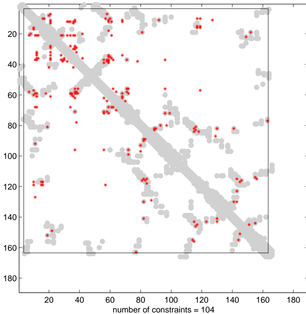
RASH_HUMAN, Residues less than 5.00 Angstroms apart
